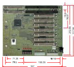
PBP-08A7 8-slot (7x PCI) Active PICMG Backplane
